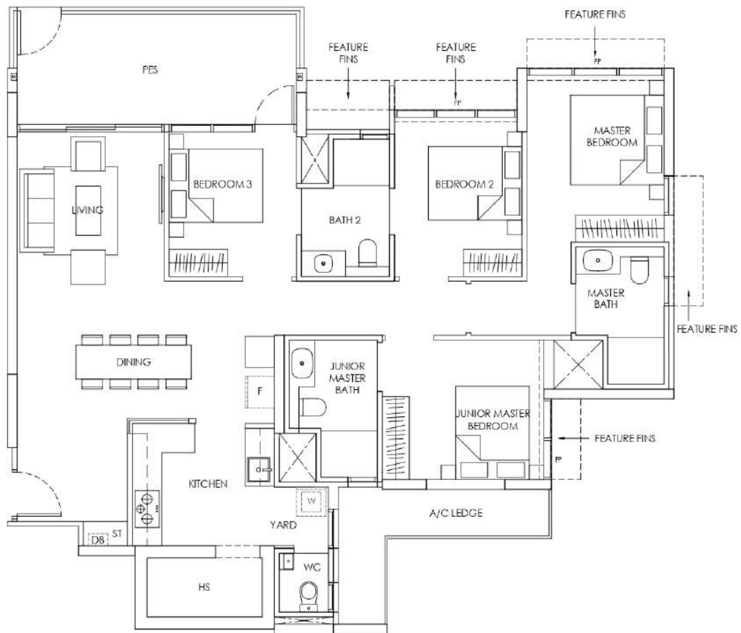
FP - FIXED WINDOW PANEL
